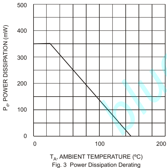
Fig. 3 Power Dissipation Derating
